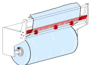
Micro-perforator kit with counter plate Modular 70
